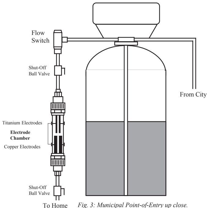
Fig. 3: Municipal Point-of-Entry up close.
